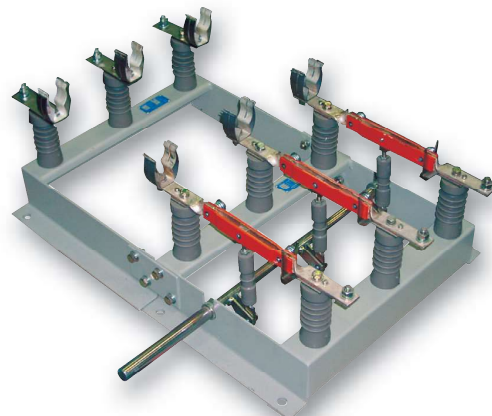
OMI with fuse base
